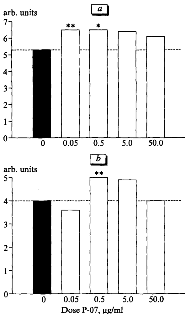
Fig. 1. Effect of hexapeptide P-07 on cytotoxic activity of human natural killers under conditions of 1-h pre-exposure and 14-h co-incubation of lymphocytes with target cells in complete nutrient medium with autologous (AS) and fetal calf serum (FCS). a ) exposure and incubation with AS ( n=4 ); b ) exposure with AS, incubation with FCS ( n=6 ); c ) exposure and incubation with FCS ( n=4 ). * p < 0.1 , ** p < 0.05 compared to the control (dark bars).
